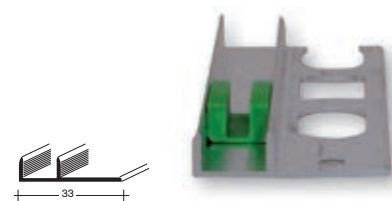
ART. 2708 - Supporto ART. 2706-2707-2714-2715-2717 Lung: m 2.70.
